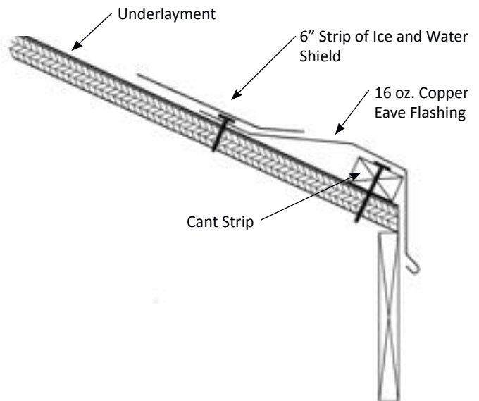
Figure 22.2 Copper Flashing Eave Detail
