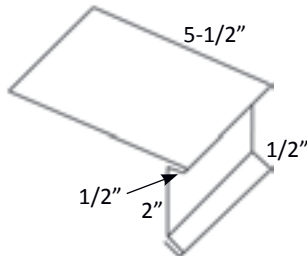
Figure 23.1 Open Rake Flashing Dimensions
