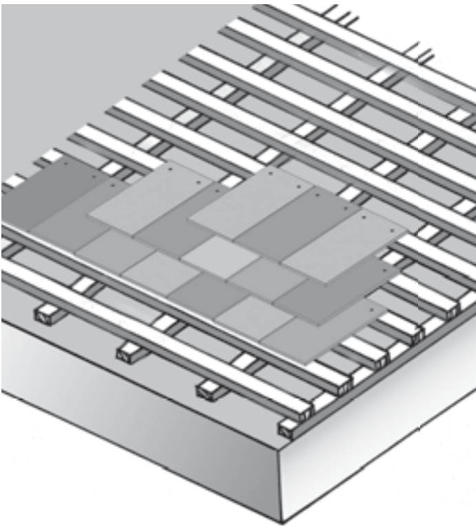
Figure 14.1 Batten System of Attachment for Concrete Deck
