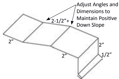
Figure 22.1 Eave Flashing Dimensions
