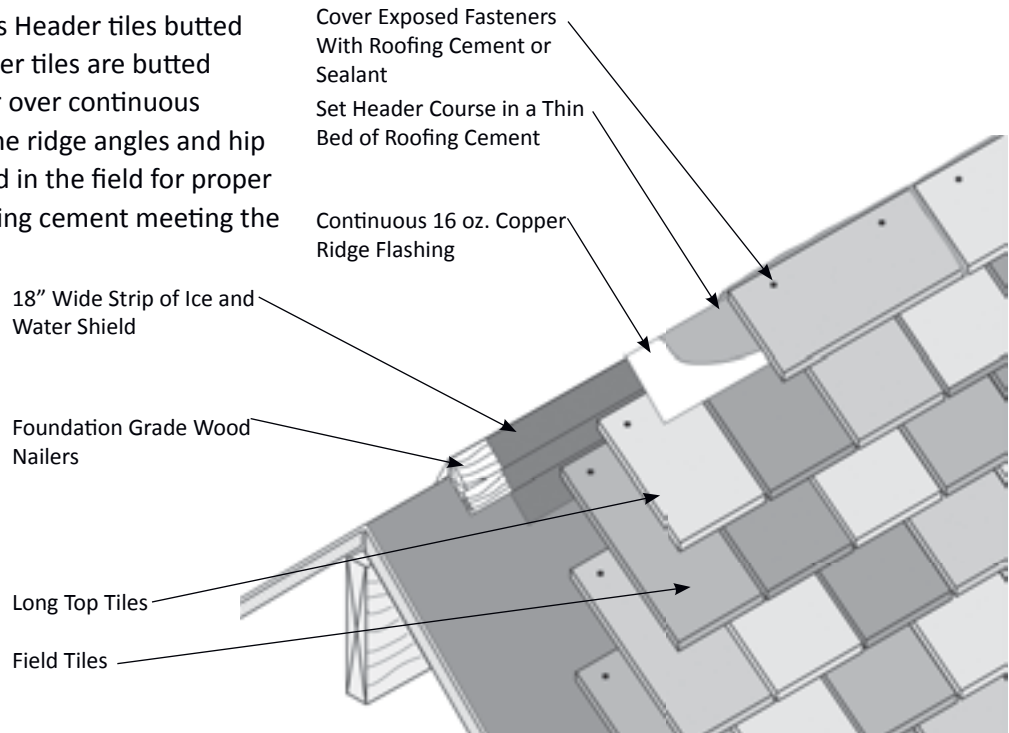
Figure 39.1 Flush Butted Header Course Ridge Detail
