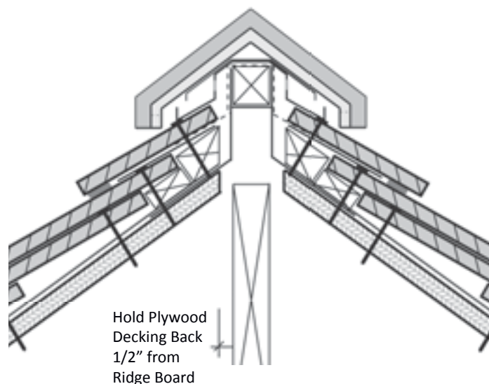
Figure 40.3 #211 Vented Ridge Section
