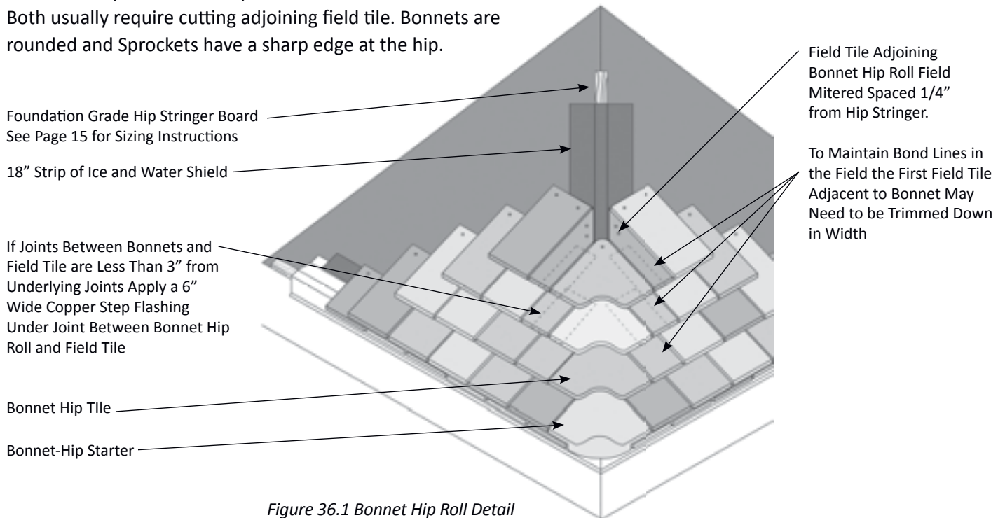
Figure 36.1 Bonnet Hip Roll Detail
