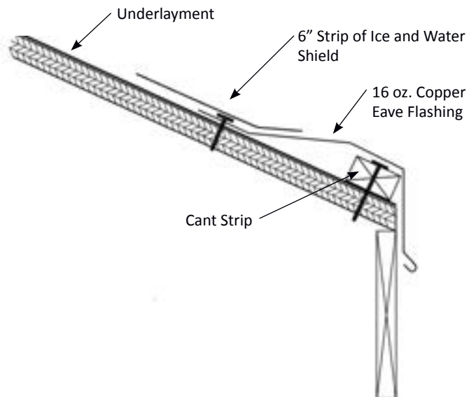
Figure 22.2 Copper Flashing Eave Detail
