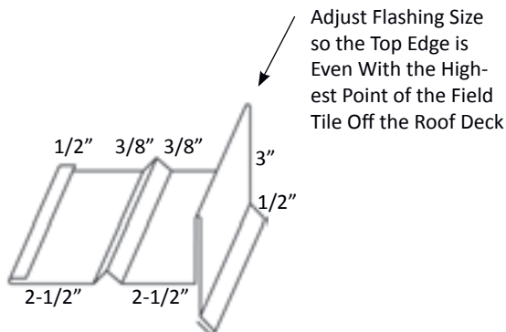
Figure 23.2 Closed Rake Flashing Dimensions
