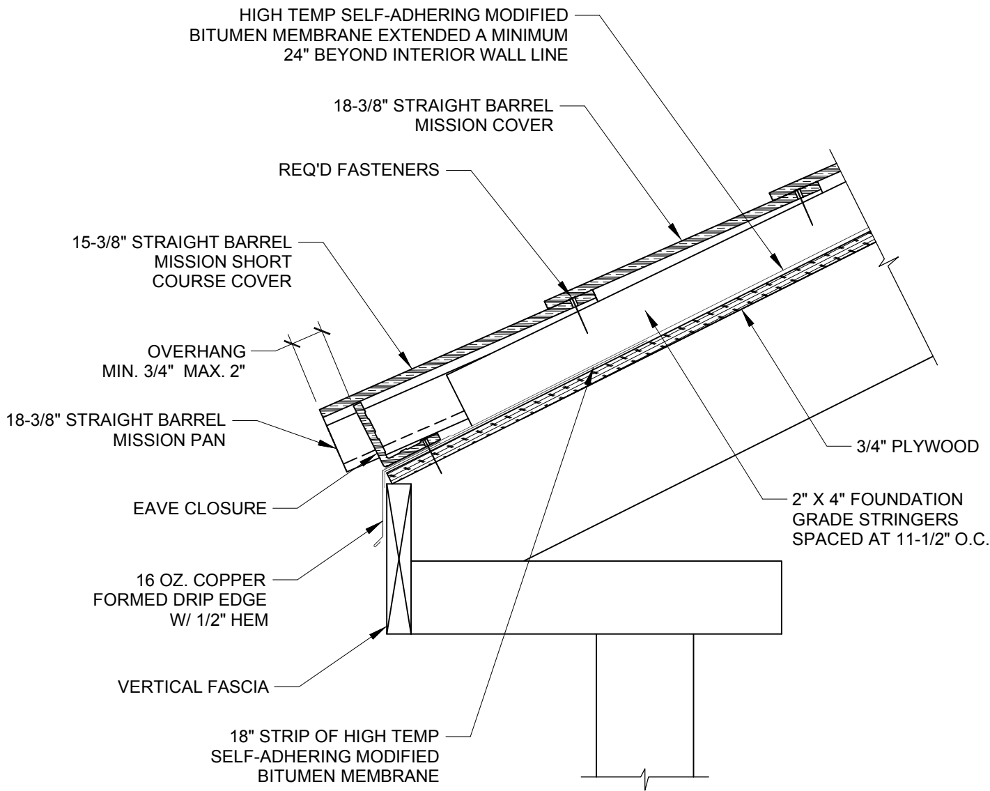
SECTION AT EAVE SCALE 1-1/2" = 1'
